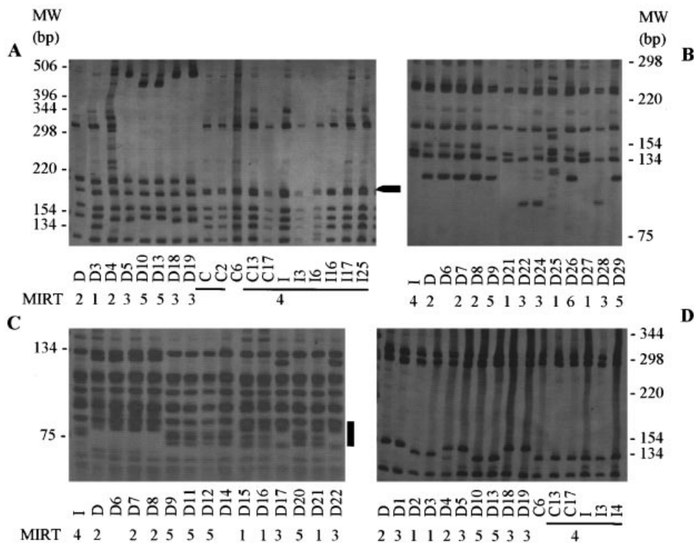
Fig. 3. Restriction profiles generated by enzymes (A) Cfo I and (B) Hae III on ITG/CS amplification products, and enzymes (C) Cfo I and (D) Msp I on ITG/L amplification products. Cfo I generated specific profiles for L. infantum / L. chagasi for band sizes indicated by an arrow upon ITG/CS and by a bar upon ITG/L. The MIRT types corresponding to each strain and restriction pattern are indicated.
